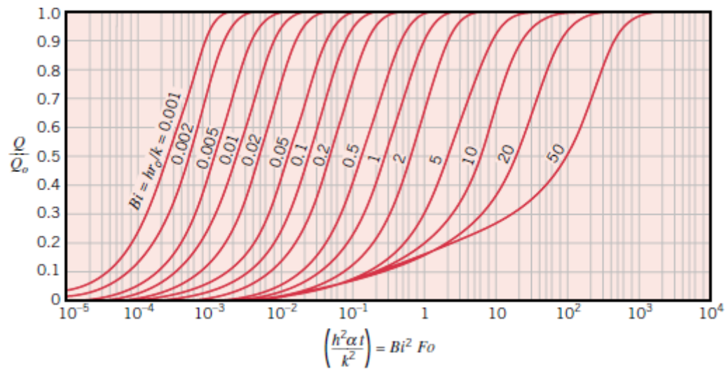
FIGURE 5S.9 Internal energy change as a function of time for a sphere of radius r_0
