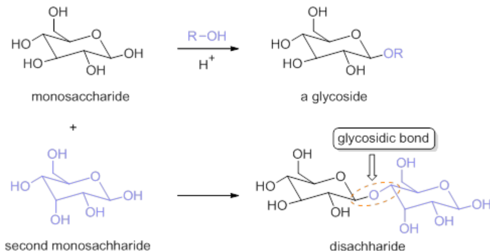
Scheme 10
