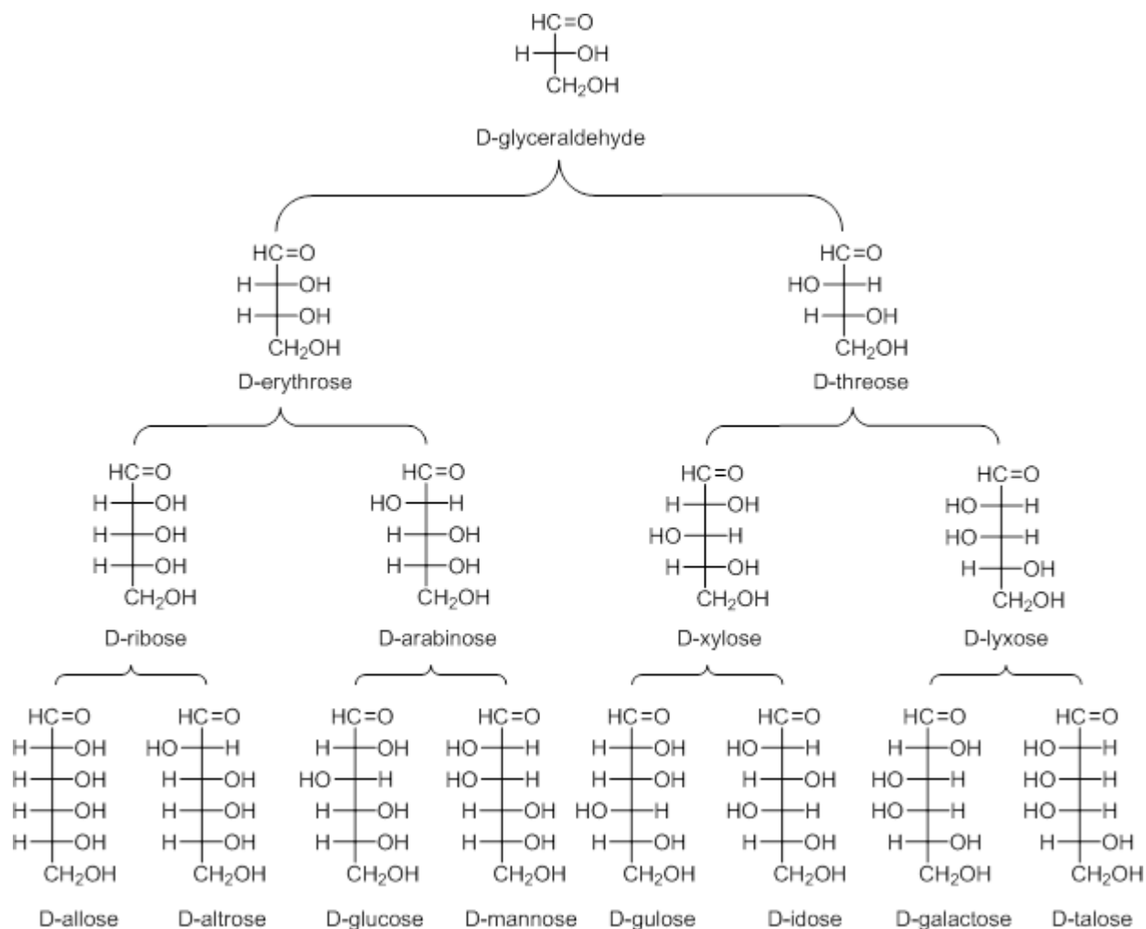
Scheme 10
