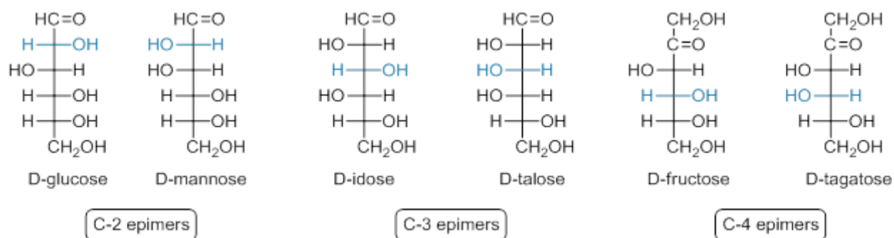
Scheme 12
