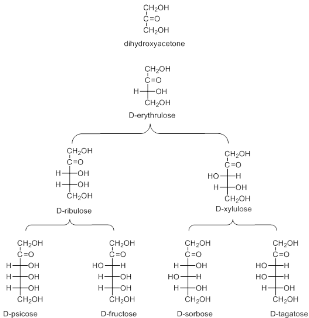
Scheme 11
