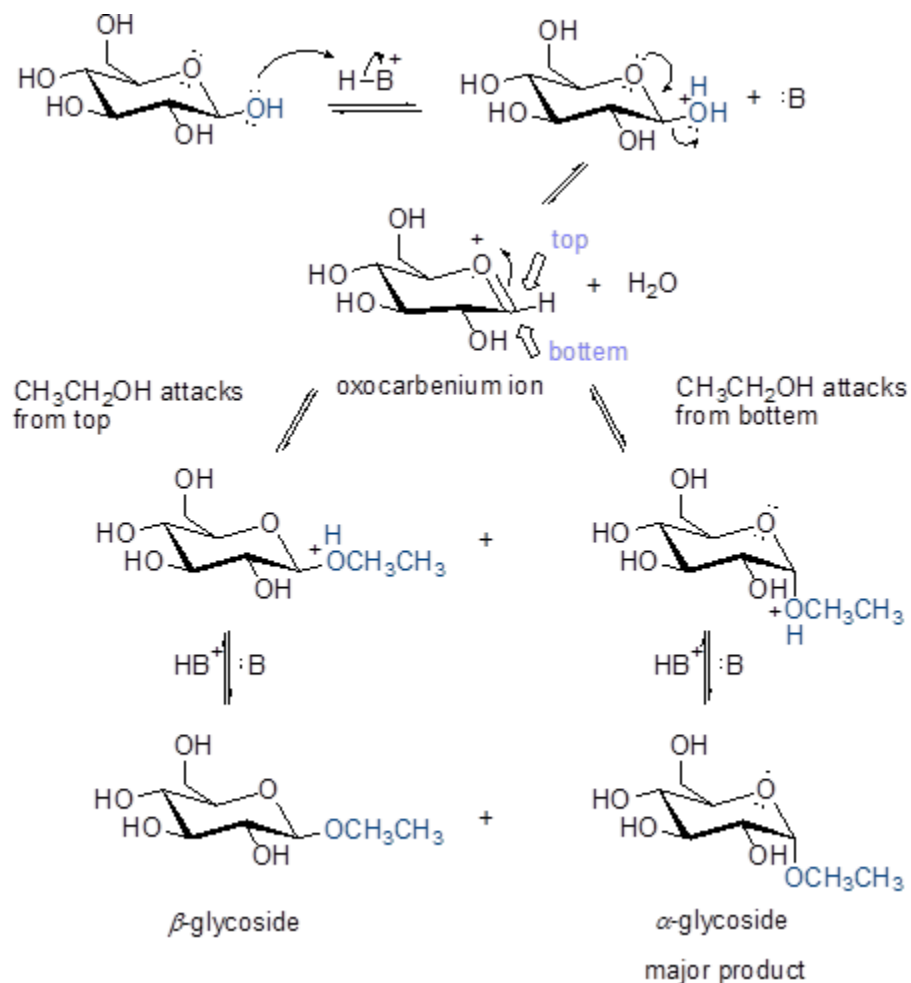
Scheme 3
