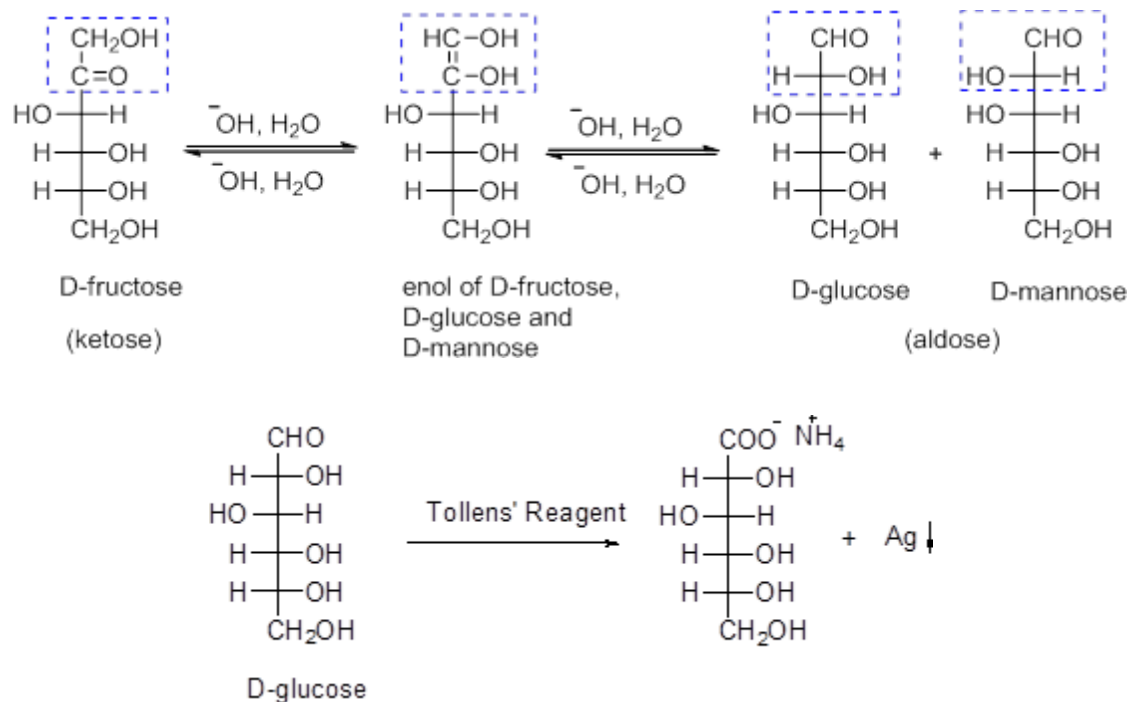
Scheme 5
