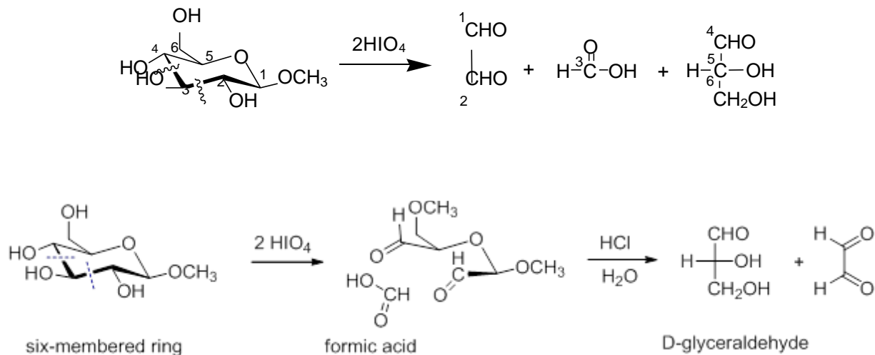
Scheme 8
