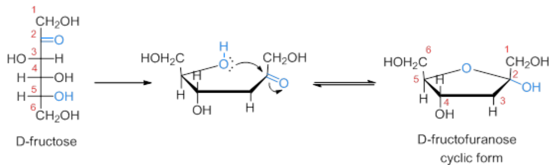
Scheme 14
